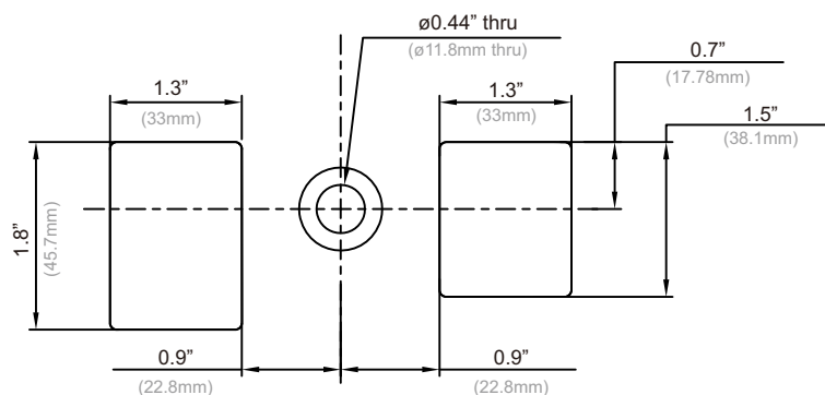
PARTIAL VIEW
