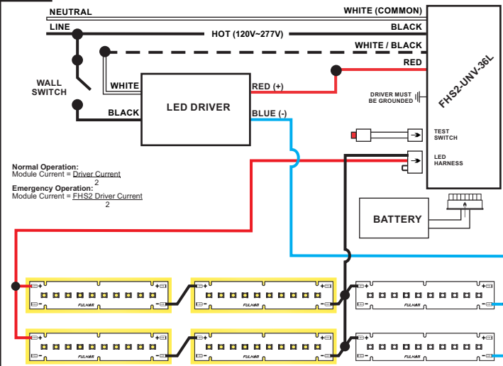
31-A Series / Parallel, Six (6) Modules, Four (4) in Emergency
