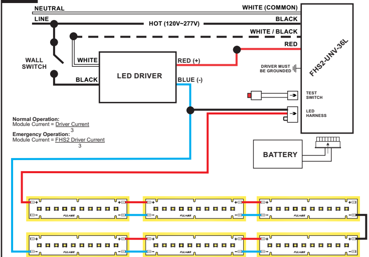
32-B Series / Parallel, Six (6) Modules, Six (6) in Emergency
