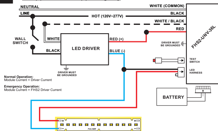
1 One (1) Module, One (1) Emergency
