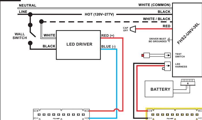
35 Two (2) Modules, One (1) in Emergency
