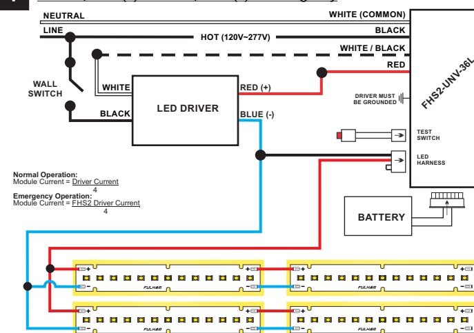
4 Parallel, Four (4) Modules, Four (4) in Emergency
