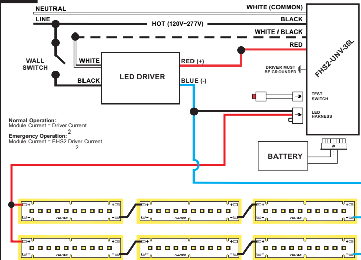
32-A Series / Parallel, Six (6) Modules, Six (6) in Emergency
