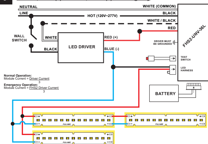
3 Parallel, three (3) Modules, Three (3) in Emergency
