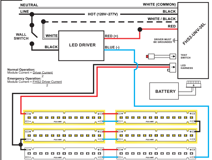
32-B Series / Parallel, Six (6) Modules, Six (6) in Emergency
