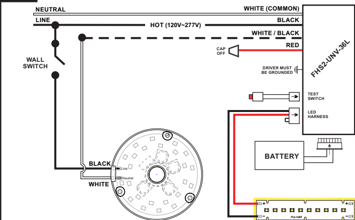
34 One (1) LED Engine, One (1) DC Module in Emergency
