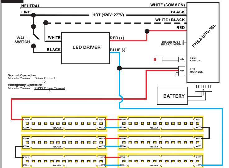
33-B Series / Parallel, Six (6) Modules, Six (6) in Emergency
