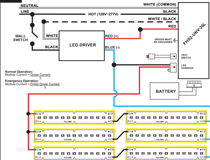
33-A Series / Parallel, Six (6) Modules, Six (6) in Emergency
