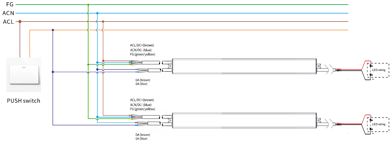
Wiring diagram
