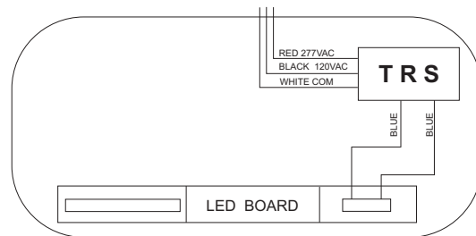
AC Only Wiring Diagram:
