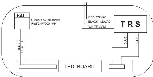
Exit Battery Wiring Diagram:
